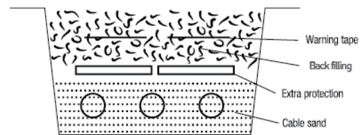
(1.2b) Three single core cables in flat formation
