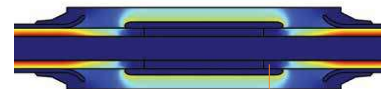
Simulations: Design based on computer FEM-simulations for optimal electrical stress.
